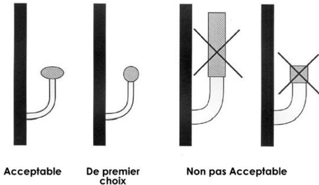
Illustration 4 - Balustrades
